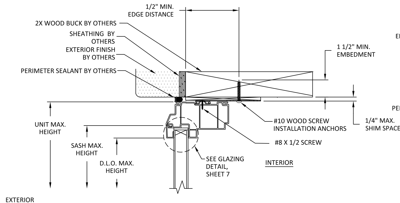
A 6 VERTICAL SECTION CLIP INSTALLATION WOOD SUBSTRATE
