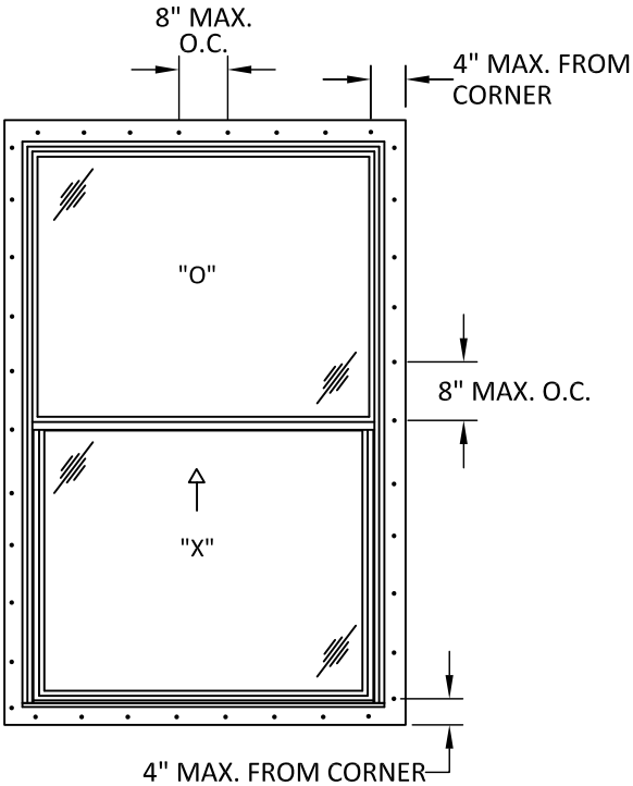
ANCHOR LAYOUT NAIL FIN INSTALLATION
